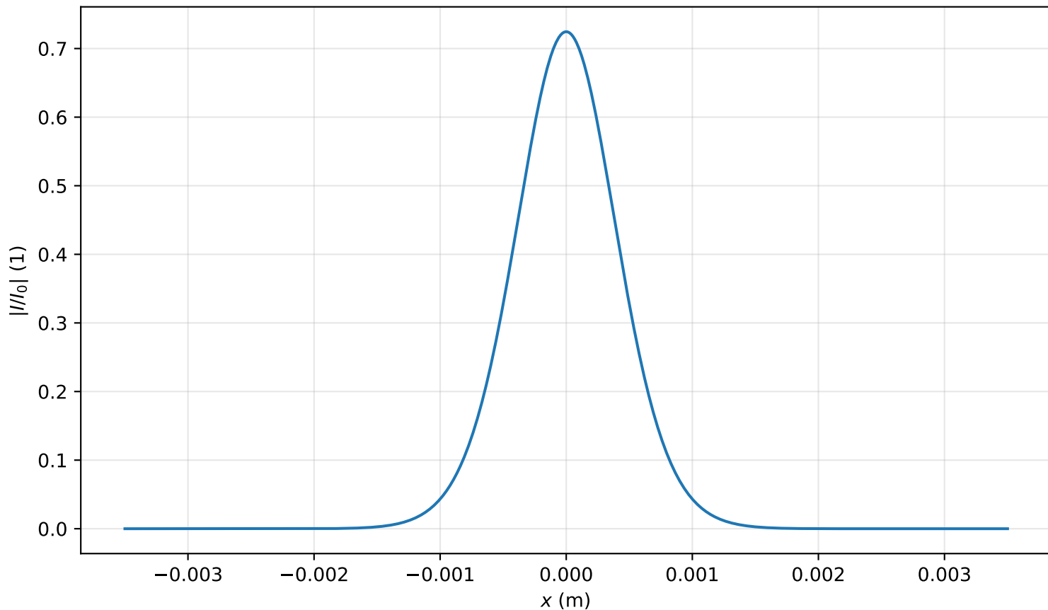
Intensity profile I(x, y = 0, z = 1.751m)/I_0 , P_{in}=0.3P_{cr} , artificial time
